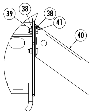
DETAIL H
