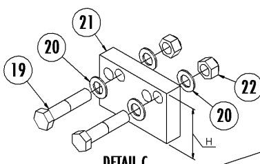
DETAIL C
