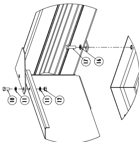
DETAIL B 1:5
